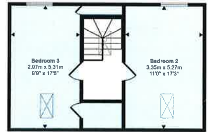
Second Floor Approx 44 sq m / 473 sq ft
